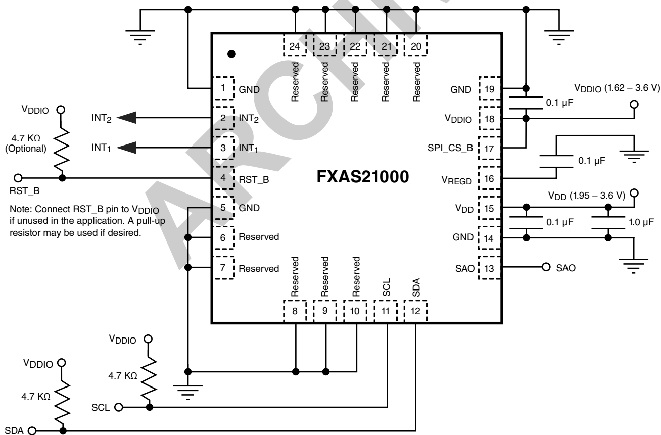
Figure 3. I 2 C mode electrical connections
