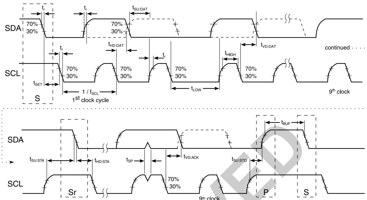
Figure 6. I²C timing diagram
